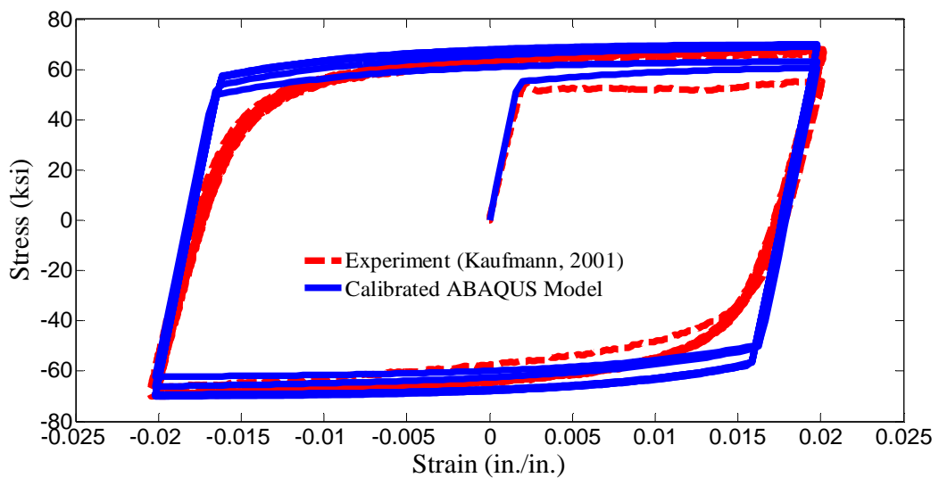
Figure 5. 4. Test data from Kaufmann (2001) and comparison with ABAQUS calibrated material model, A572 Gr. 50 steel.
