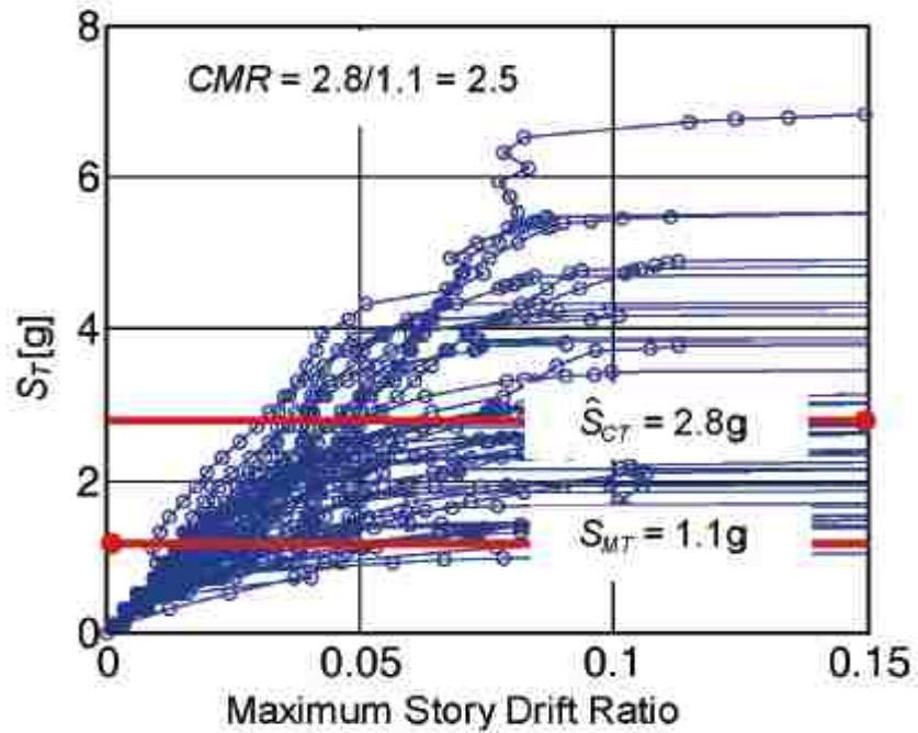
Figure 7. 1. Incremental dynamic analysis response plot of spectral acceleration versus maximum story drift ratio (FEMA P695).
