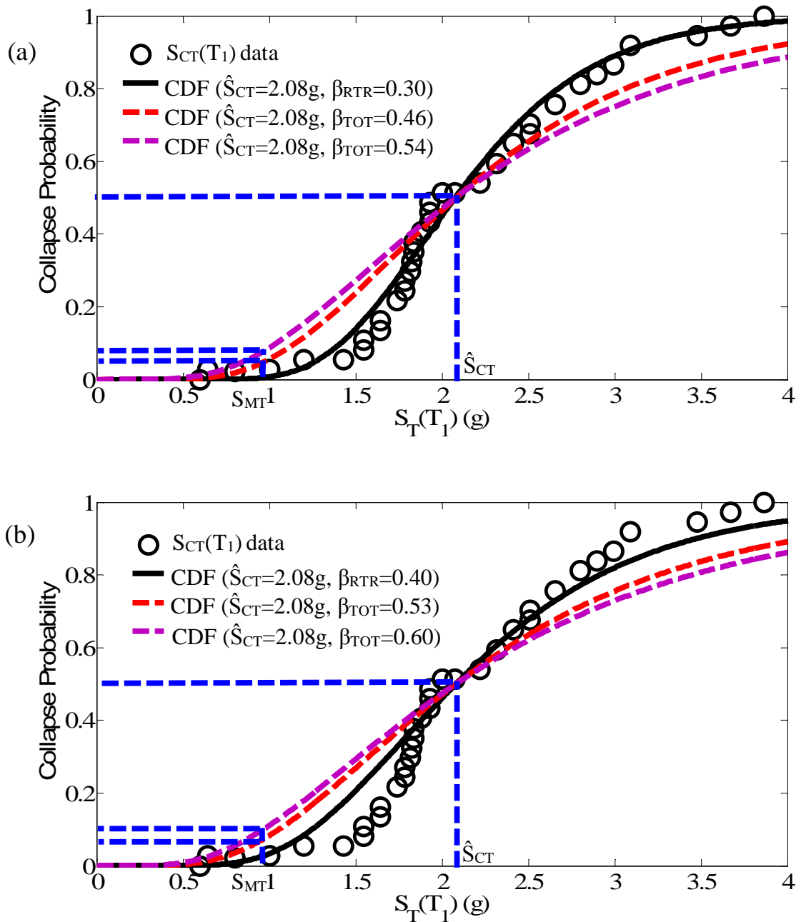
Figure 9. 7. SMRF: (a) collapse fragility curves using \beta_{RTR}=0.3 ; (b) collapse fragility curves using \beta_{RTR}=0.4 ; S_{CT}(T_1) based on minimum of S_T(T_1) at incipient collapse and at which an 80% slope reduction in the initial slope of the IDA curve takes place, far-field ground motions.
