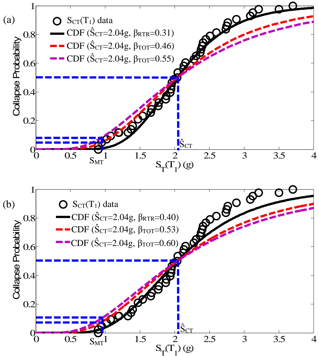
Figure 8. 13. SC-MRF Design 1: (a) collapse fragility curves using \beta_{RTR}=0.31 ; (b) collapse fragility curves using \beta_{RTR}=0.4 ; S_{CT}(T_1) based on minimum of S_T(T_1) at incipient collapse and 10% maximum story drift, far-field ground motions.
