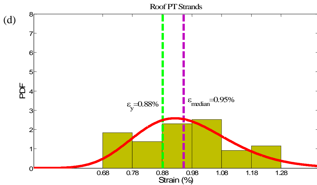
Figure 8. 16. Frequency distribution plots and PDFs of PT strand maximum strain \epsilon_{\text{max}} : (a) 1 st floor, (b) 2 nd floor, (c) 3 rd floor, and (d) Roof for SC-MRF Design 1, far-field ground motions.
