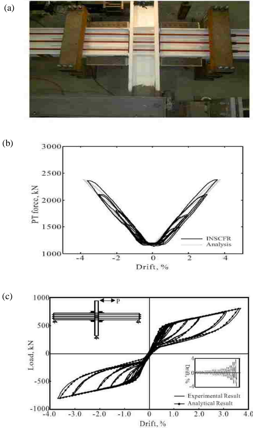
Figure 2. 8. Test by Kim and Christopoulos: (a) Test setup; (b) PT force variation; (c) load-drift relation (Kim and Christopoulos (2008)).
