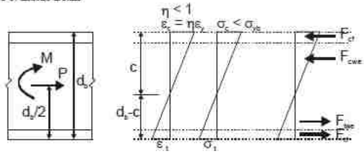
(a) Case 1: Elastic Beam
