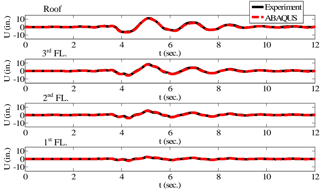
Figure 6. 6. Comparison of floor displacement time history of experimental data with ABAQUS model results under DBE for LOS000 ground motion.
